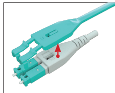
Step 2: Extract the latch from Uniboot
