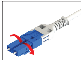
Step 3: Rotate plugs outward 180°
