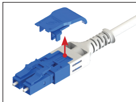
Step 2: Extract the latch from Uniboot
