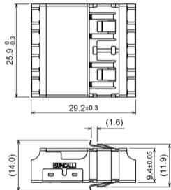
QUAD VERTICAL SPRING
